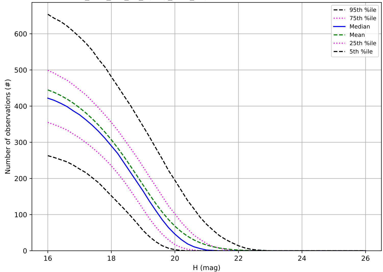
too_elab_r64_d2_ugrizy_v3.4_10yrs: Number of observations MBA
