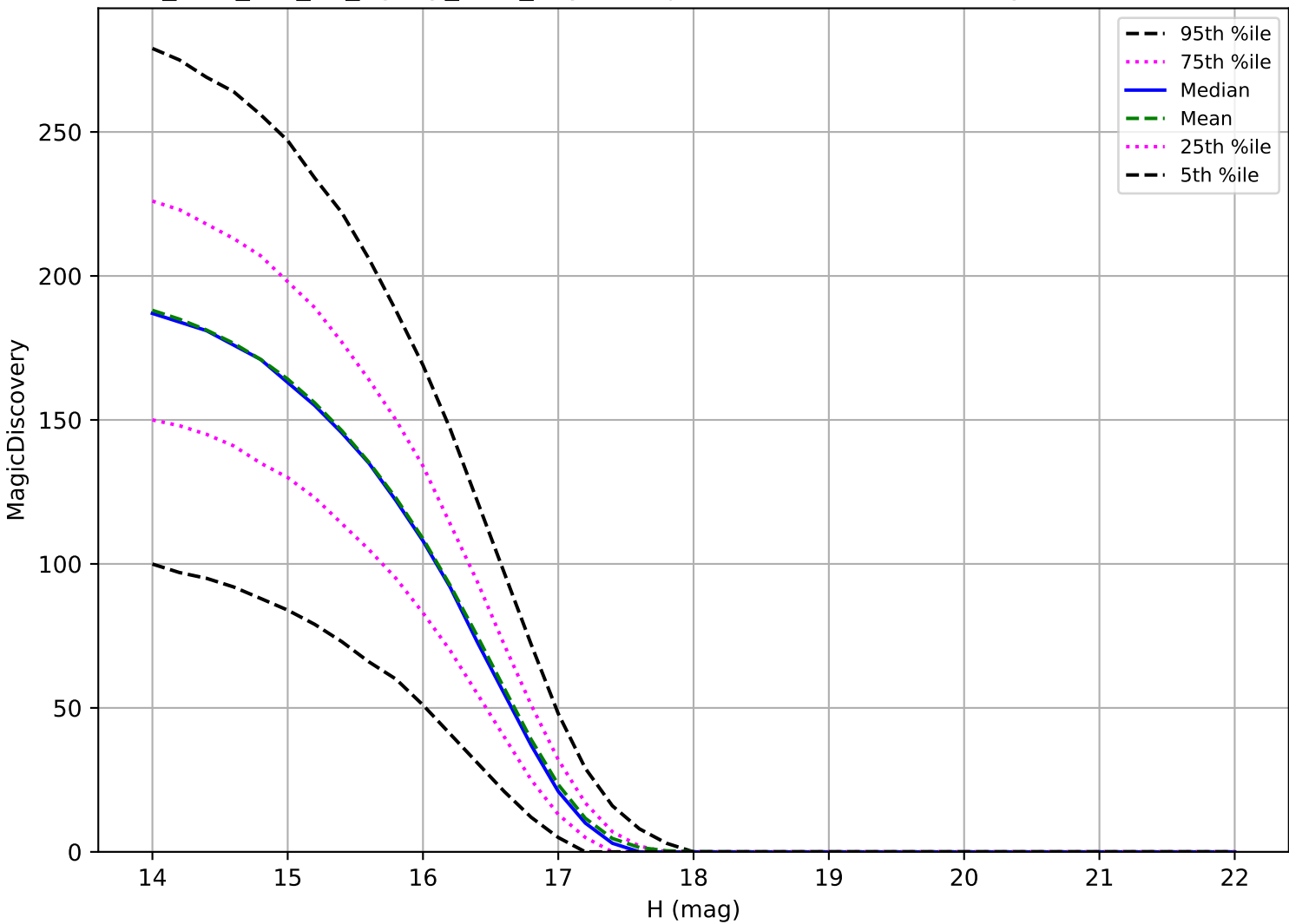
too_elab_r64_d2_ugrizy_v3.4_10yrs: Trojan 6 detections in 60 nights detection loss
