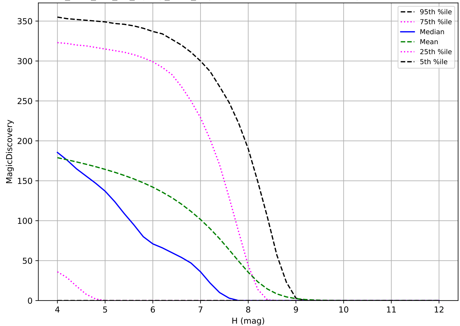
too_elab_r64_d2_ugrizy_v3.4_10yrs: TNO 6 detections in 60 nights detection loss
