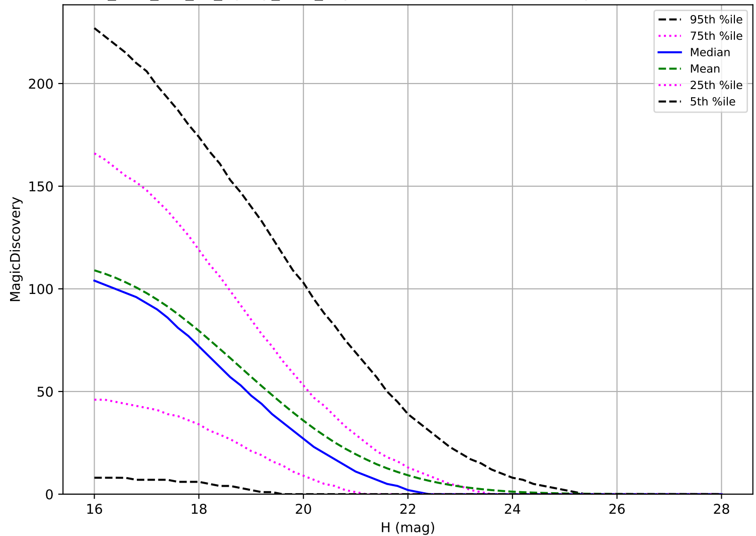
too_elab_r64_d2_ugrizy_v3.4_10yrs: PHA 6 detections in 60 nights detection loss
