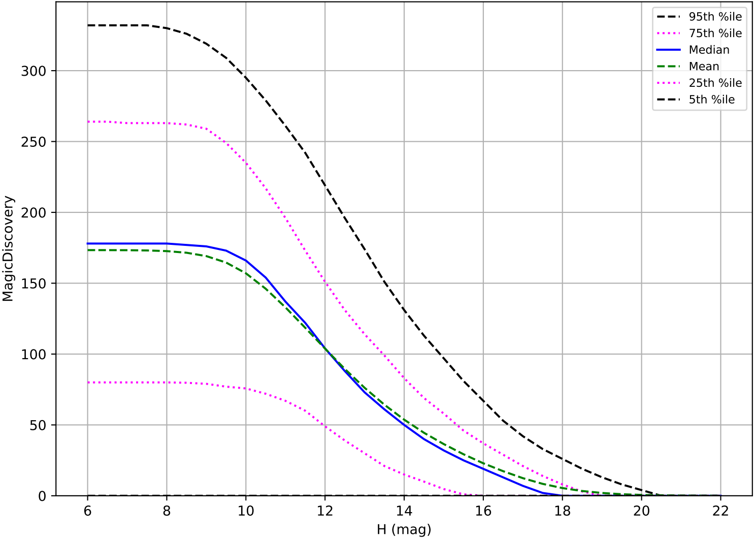
too_elab_r64_d2_ugrizy_v3.4_10yrs: OCC_r5 6 detections in 60 nights detection loss
