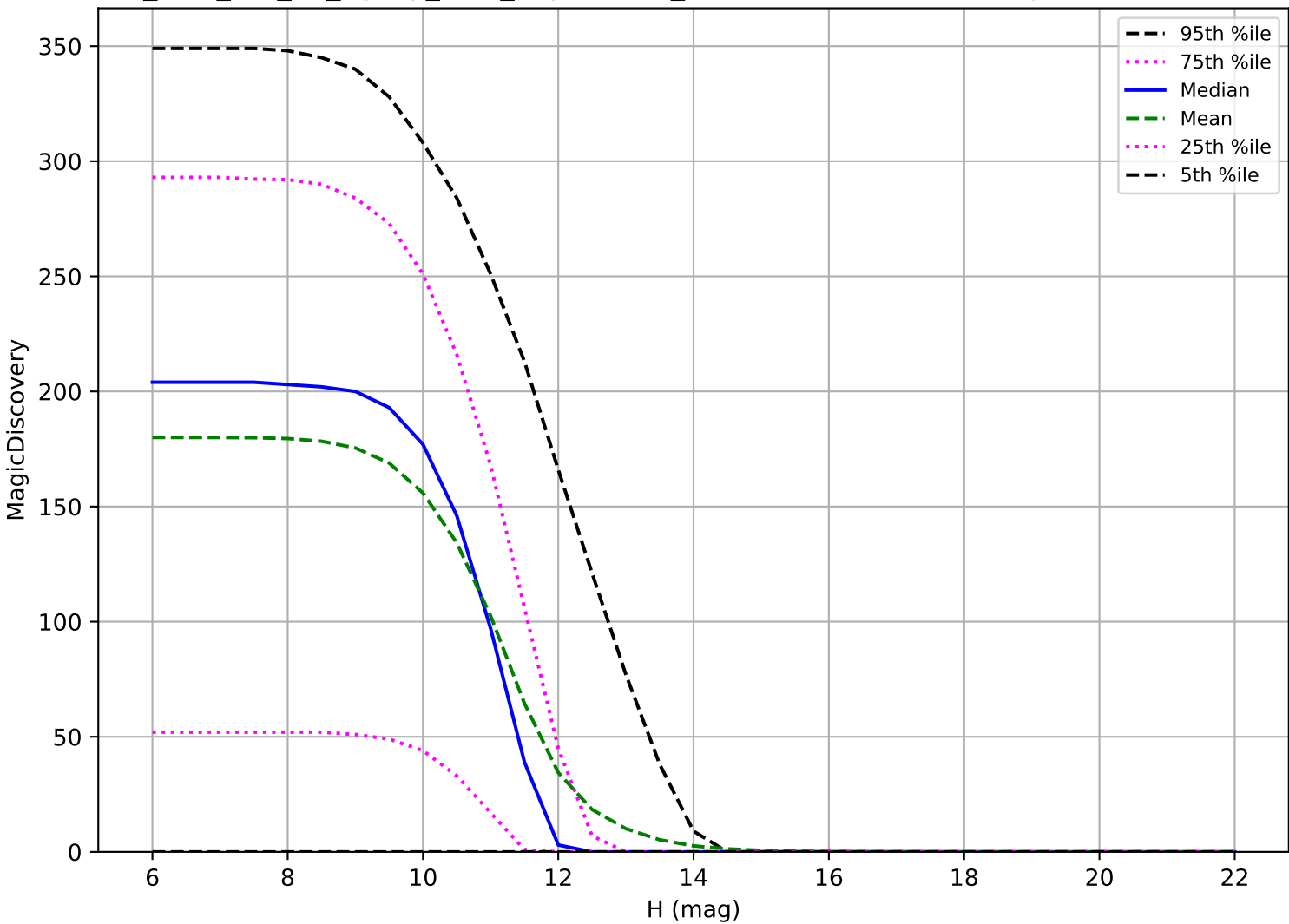
too_elab_r64_d2_ugrizy_v3.4_10yrs: OCC_r20 6 detections in 60 nights detection loss
