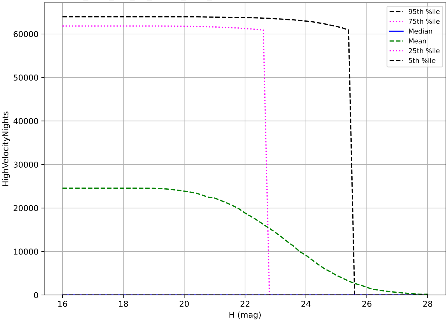
too_elab_r64_d2_ugrizy_v3.4_10yrs: PHA High velocity pair detection loss
