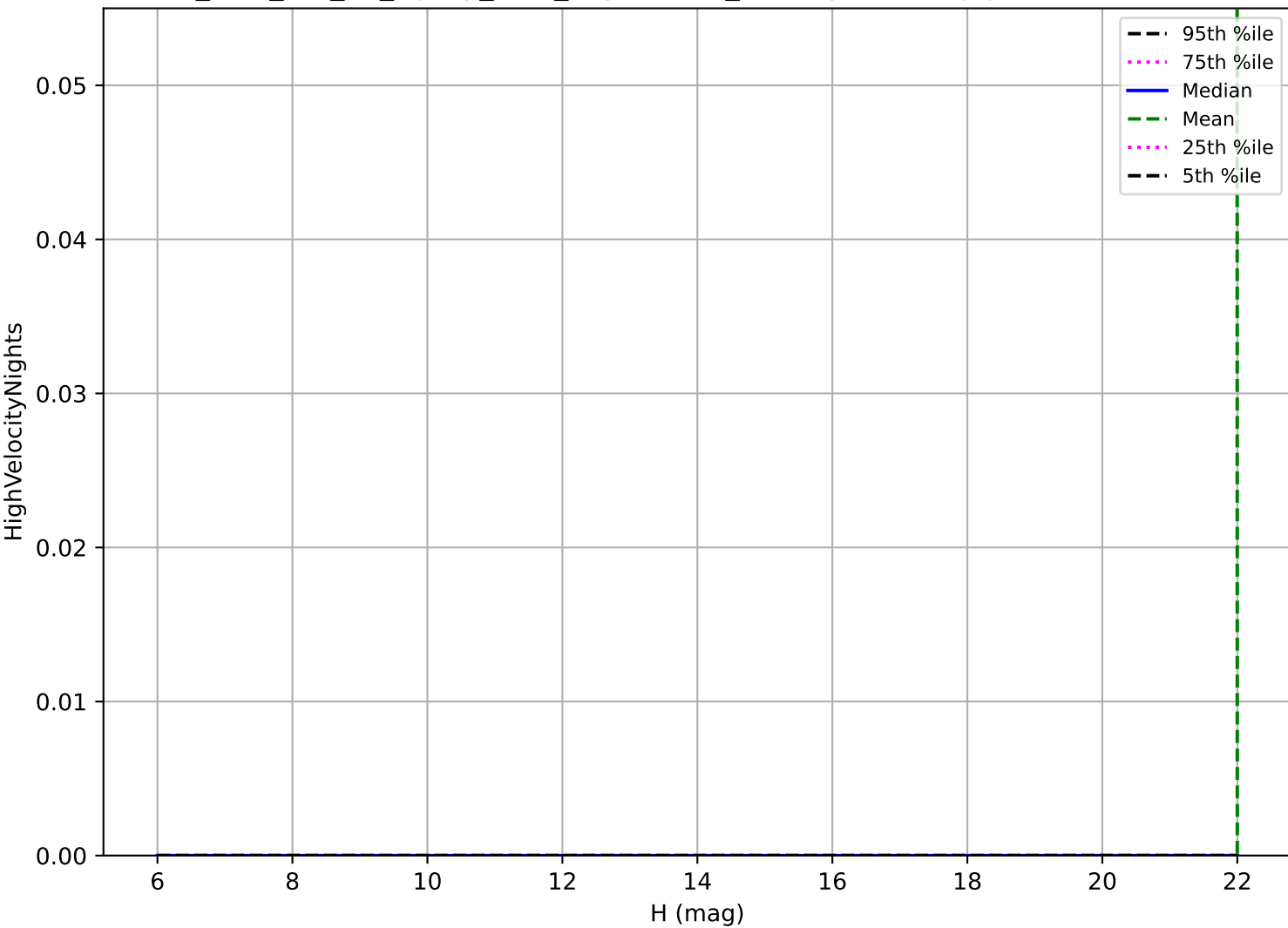
too_elab_r64_d2_ugrizy_v3.4_10yrs: OCC_r20 High velocity pair detection loss
