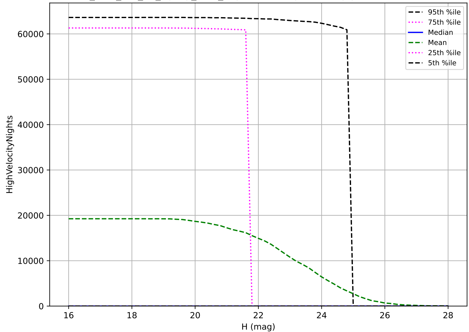
too_elab_r64_d2_ugrizy_v3.4_10yrs: NEO High velocity pair detection loss
