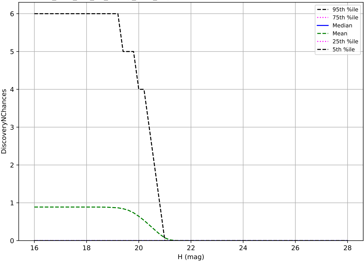
too_elab_r64_d2_ugrizy_v3.4_10yrs: Vatira 3 pairs in 15 nights detection loss
