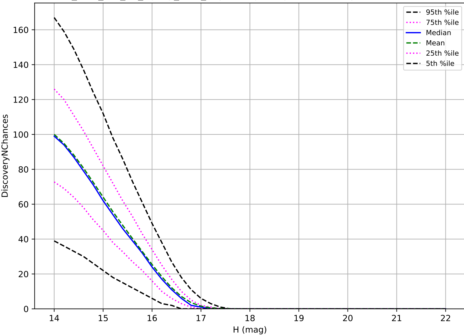
too_elab_r64_d2_ugrizy_v3.4_10yrs: Trojan 3 pairs in 15 nights detection loss
