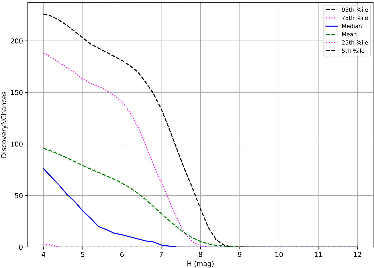
too_elab_r64_d2_ugrizy_v3.4_10yrs: TNO 3 pairs in 15 nights detection loss
