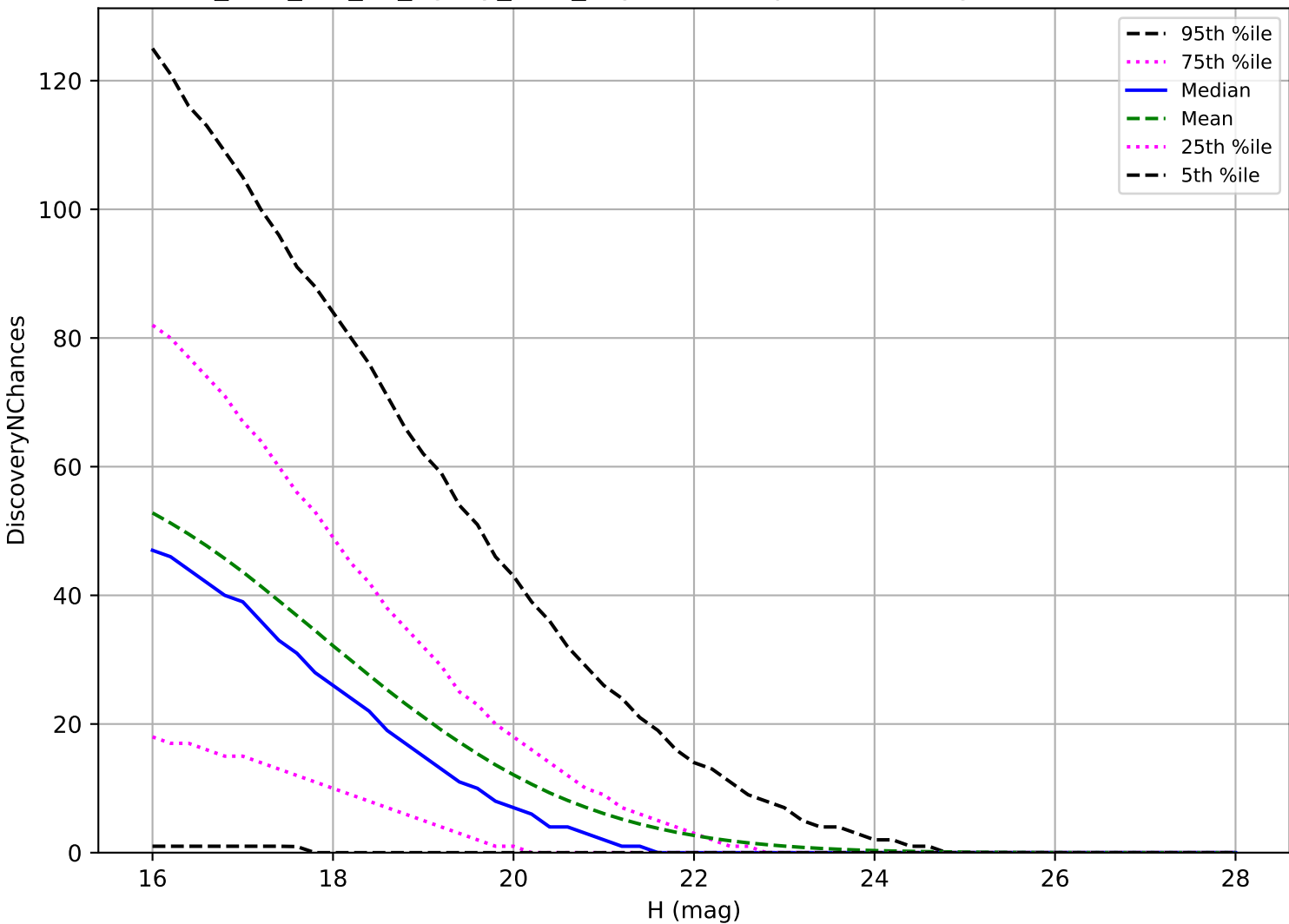
too_elab_r64_d2_ugrizy_v3.4_10yrs: PHA 3 pairs in 15 nights detection loss
