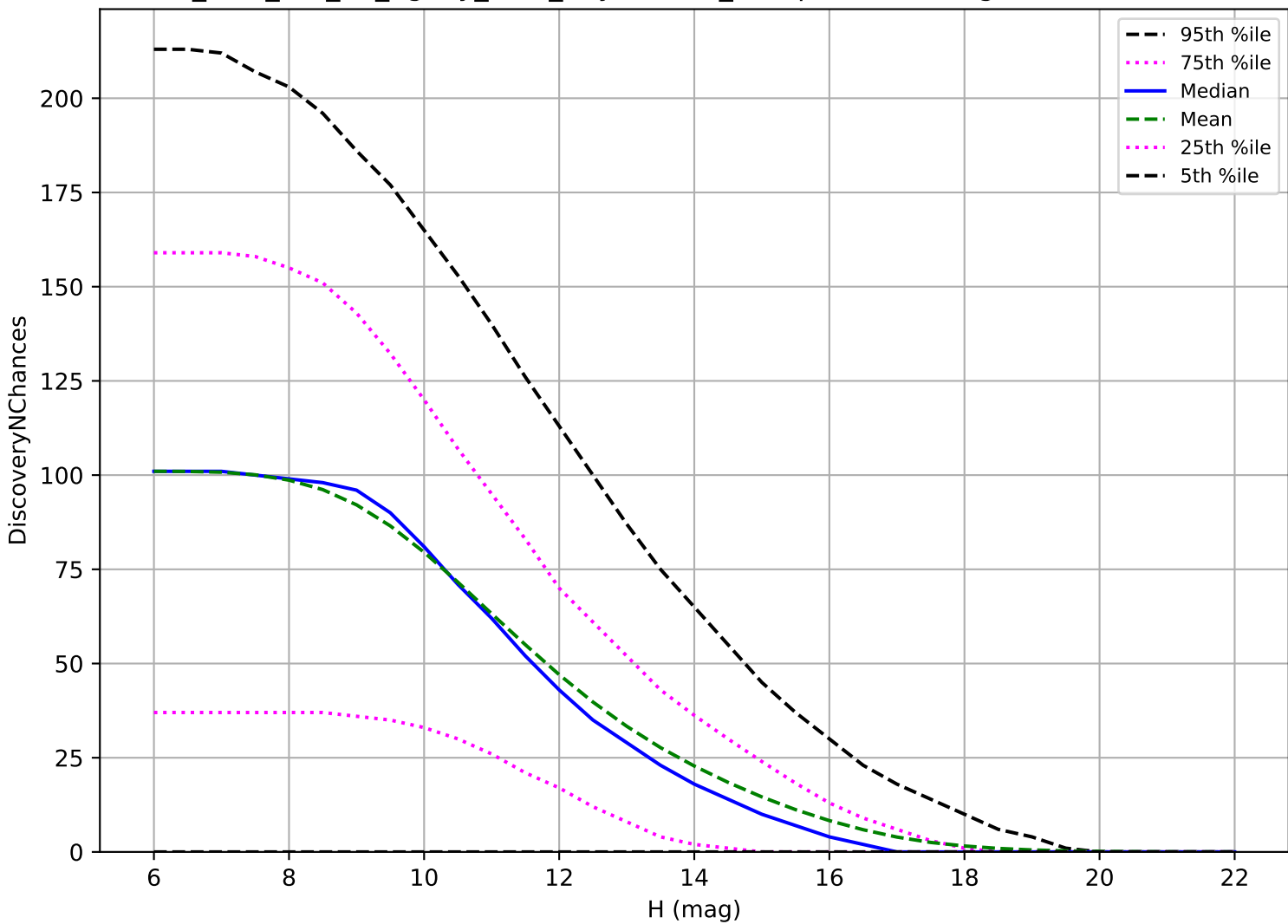
too_elab_r64_d2_ugrizy_v3.4_10yrs: OCC_r5 3 pairs in 15 nights detection loss
