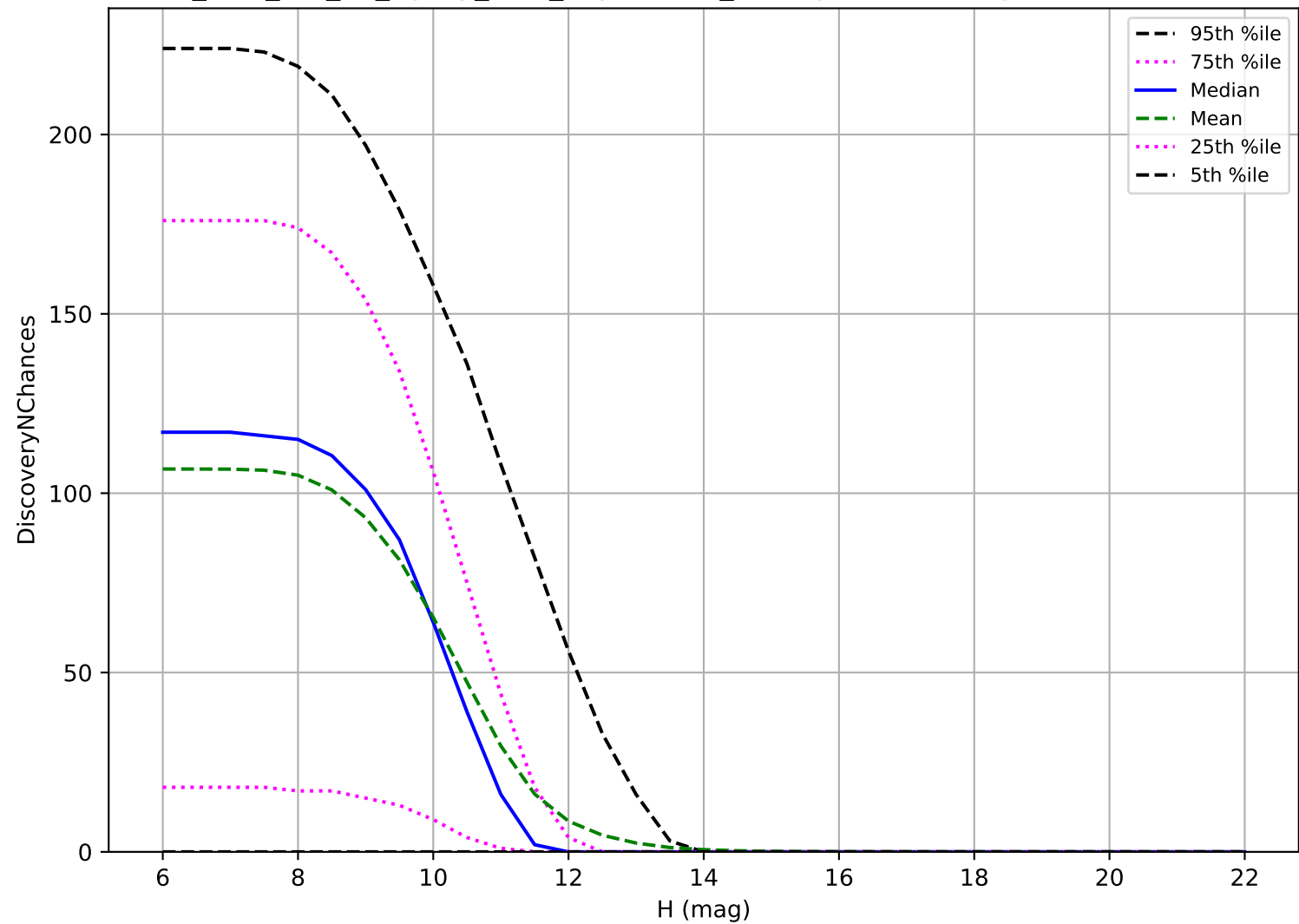
too_elab_r64_d2_ugrizy_v3.4_10yrs: OCC_r20 3 pairs in 15 nights detection loss
