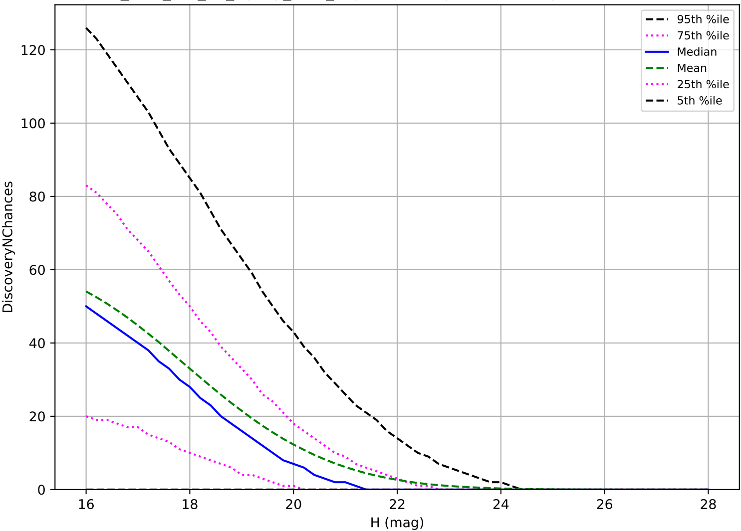
too_elab_r64_d2_ugrizy_v3.4_10yrs: NEO 3 pairs in 15 nights detection loss
