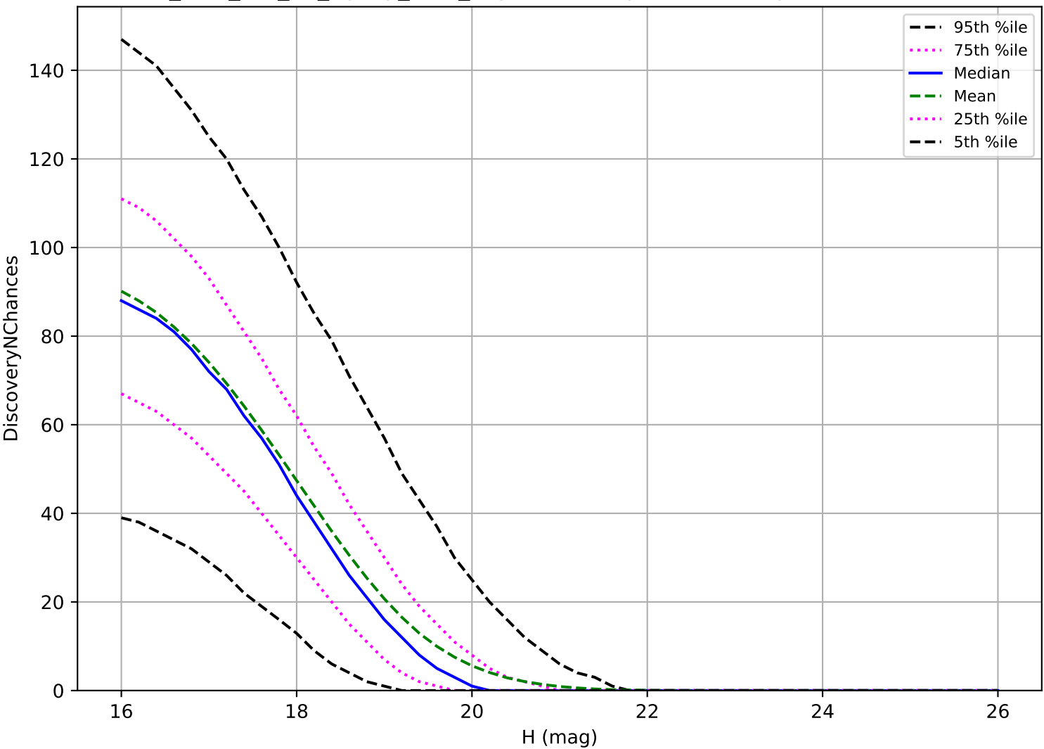
too_elab_r64_d2_ugrizy_v3.4_10yrs: MBA 3 pairs in 15 nights detection loss
