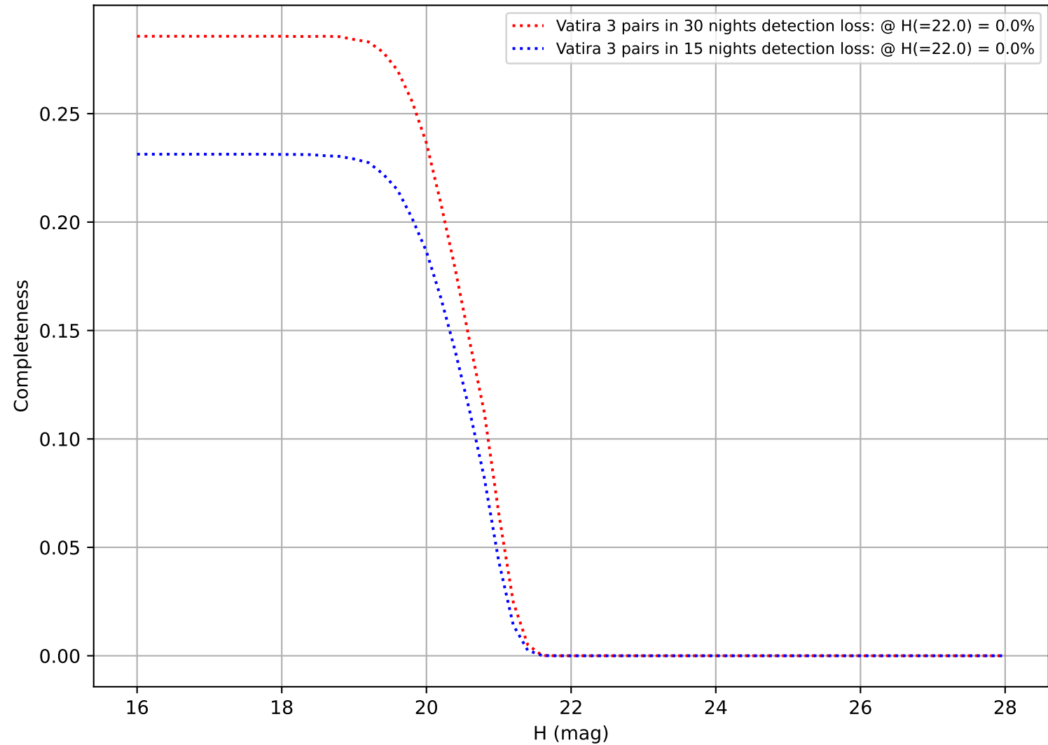
too_elab_r64_d2_ugrizy_v3.4_10yrs: DifferentialCompleteness
