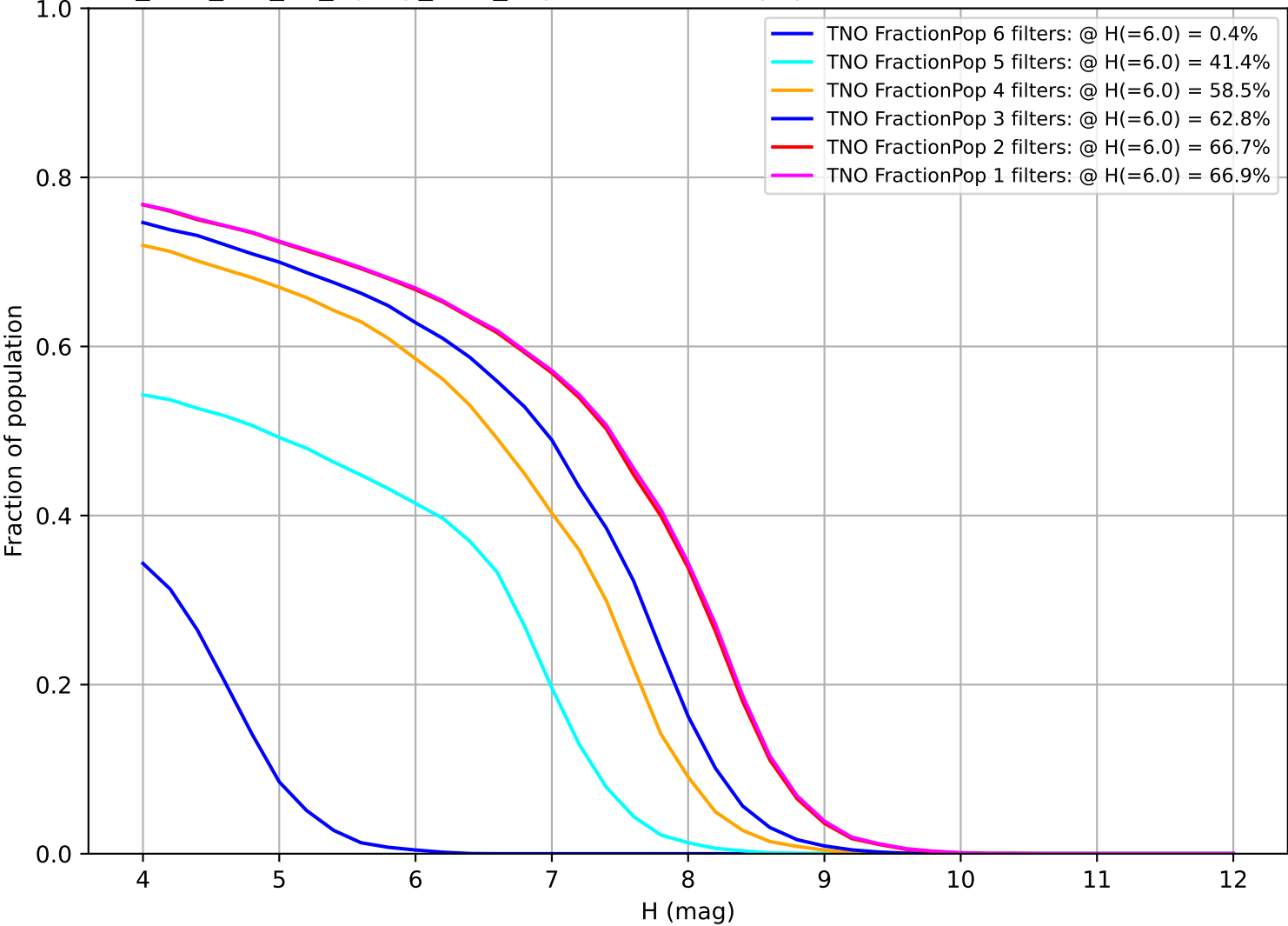
too_elab_r64_d2_ugrizy_v3.4_10yrs: Fraction of population with colors in X filters TNO
