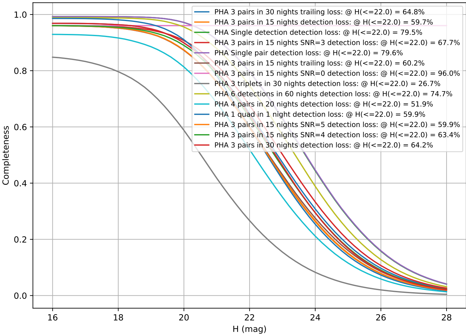
too_elab_r64_d2_ugrizy_v3.4_10yrs: CumulativeCompleteness
