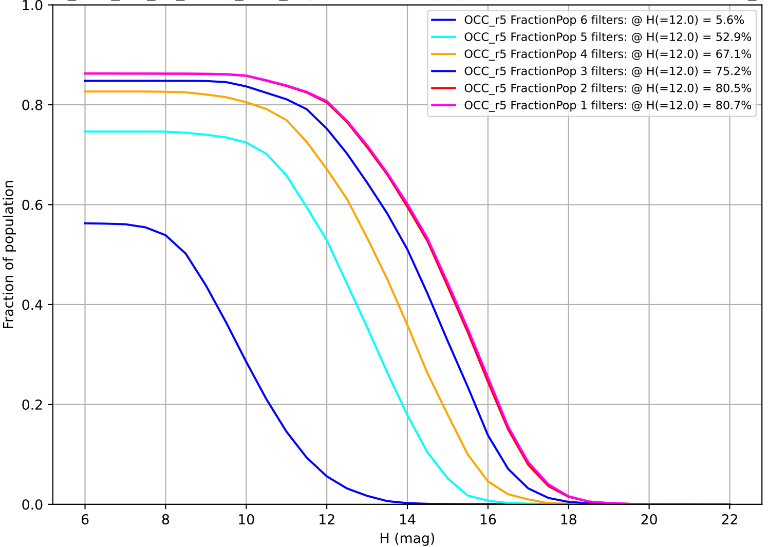
too_elab_r64_d2_ugrizy_v3.4_10yrs: Fraction of population with colors in X filters OCC_r5
