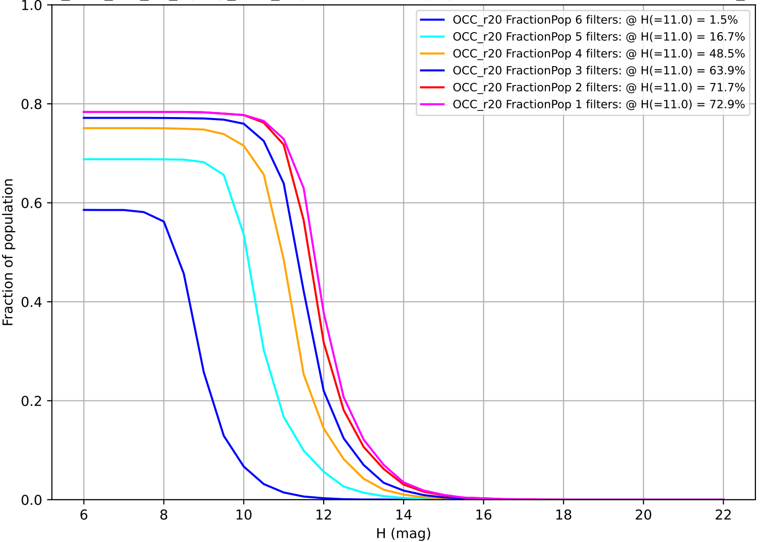
too_elab_r64_d2_ugrizy_v3.4_10yrs: Fraction of population with colors in X filters OCC_r20
