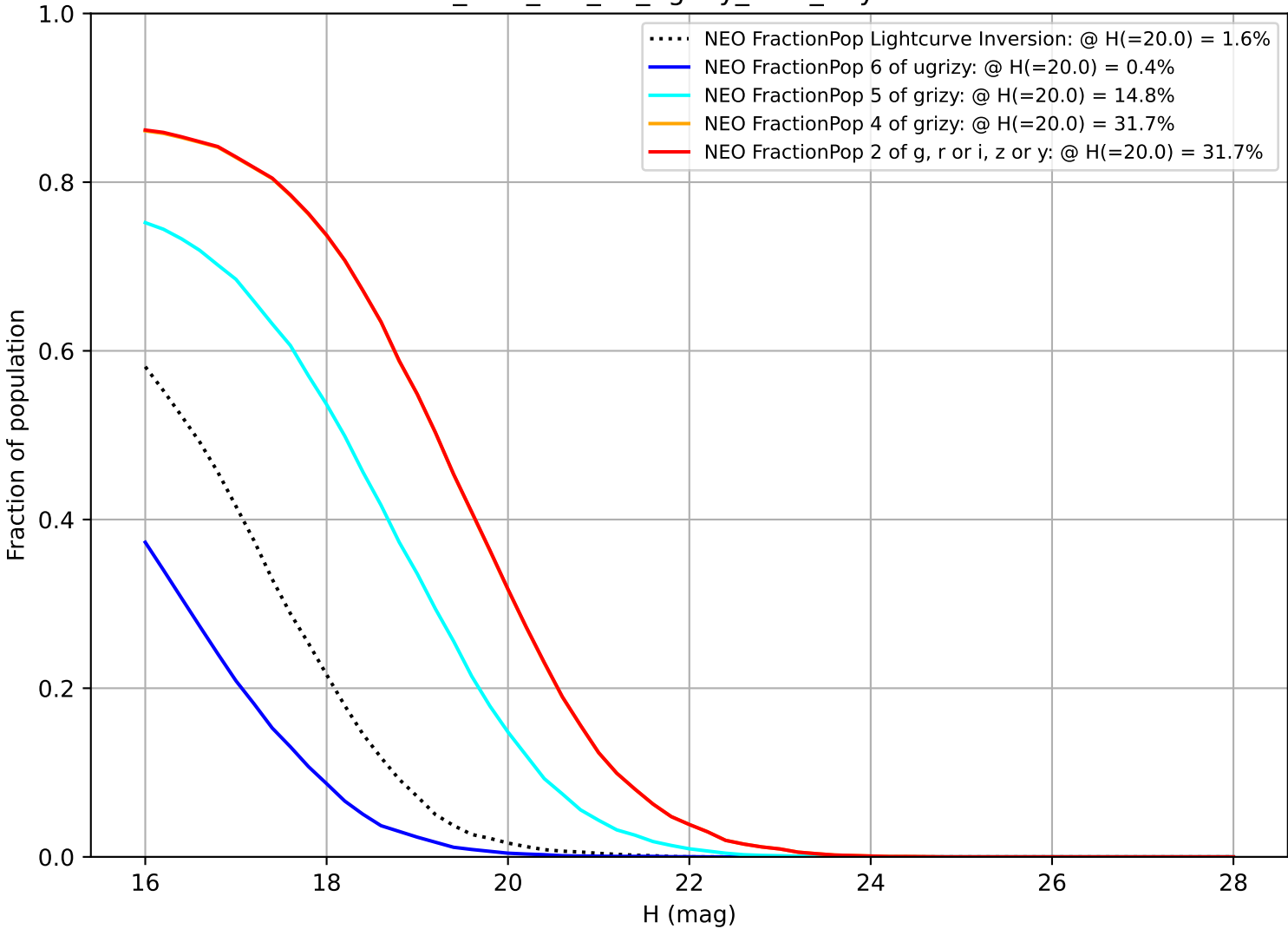
too_elab_r64_d2_ugrizy_v3.4_10yrs NEO
