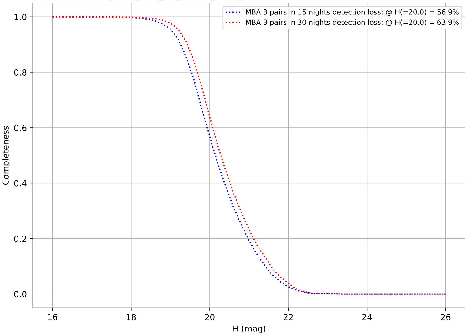
too_elab_r64_d2_ugrizy_v3.4_10yrs: DifferentialCompleteness
