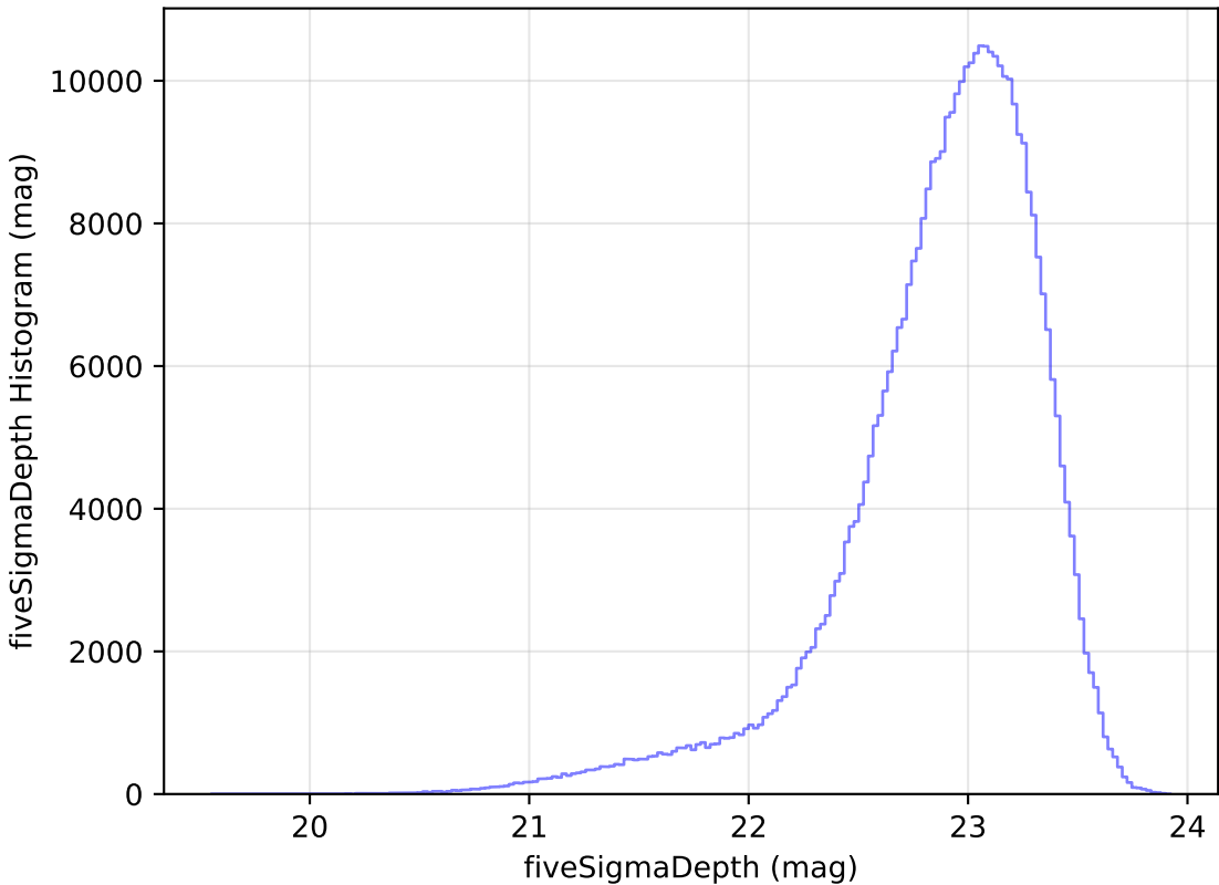
too_elab_r64_d2_ugrizy_v3.4_10yrs z: fiveSigmaDepth Histogram
