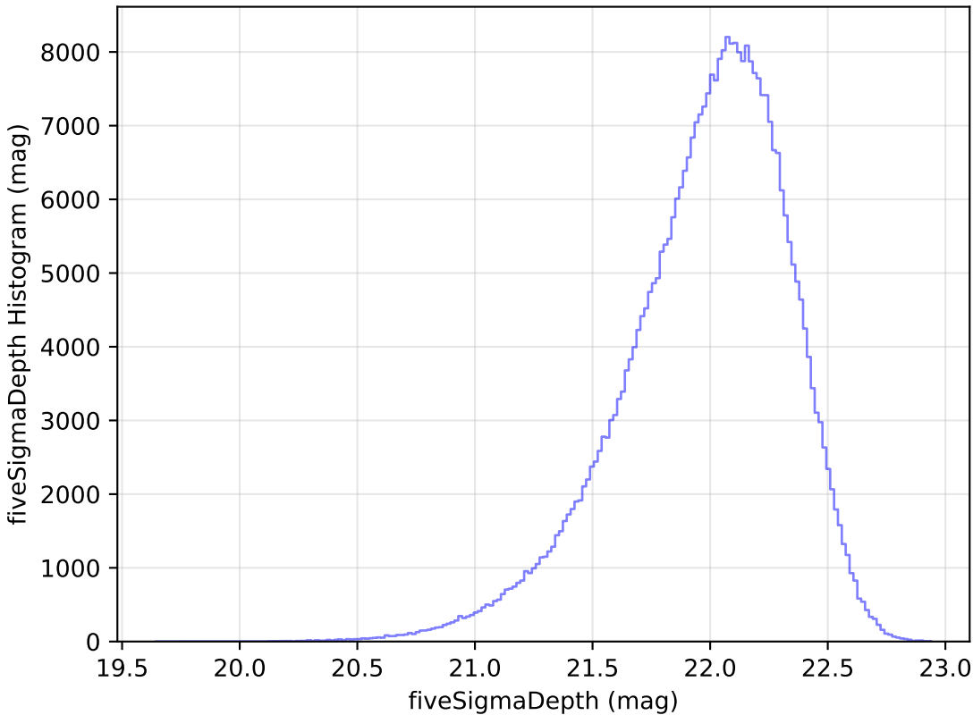
too_elab_r64_d2_ugrizy_v3.4_10yrs y: fiveSigmaDepth Histogram
