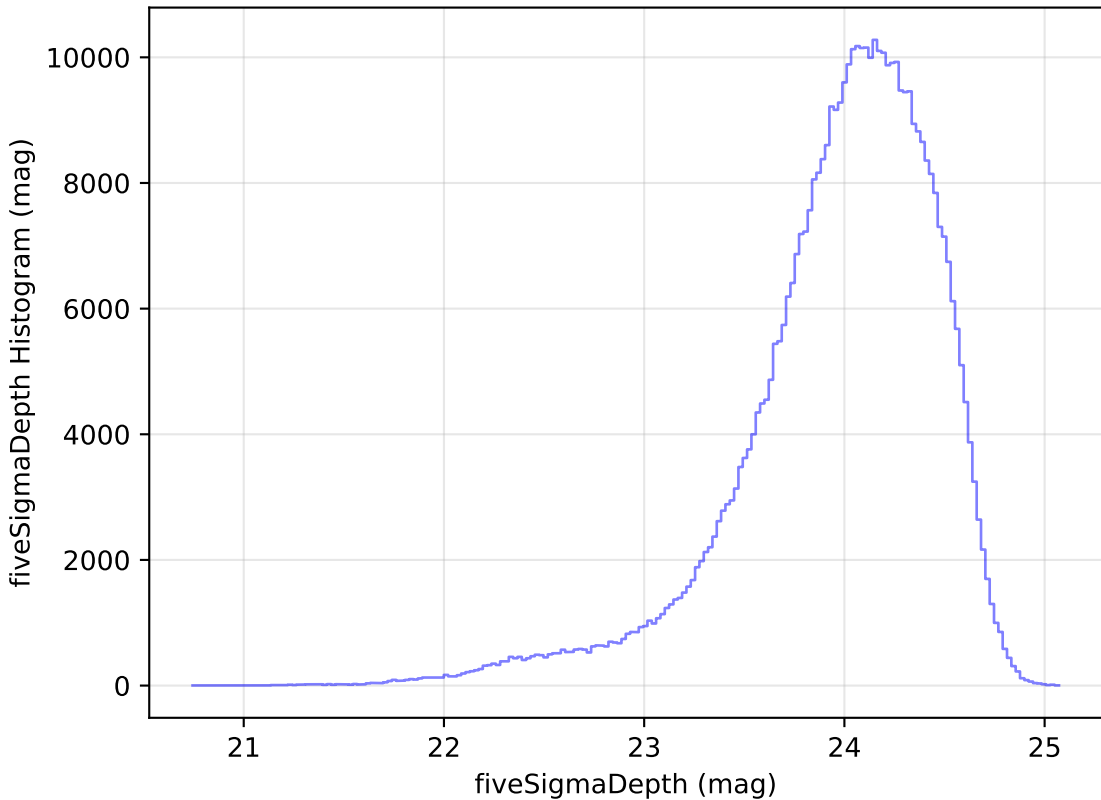
too_elab_r64_d2_ugrizy_v3.4_10yrs r: fiveSigmaDepth Histogram
