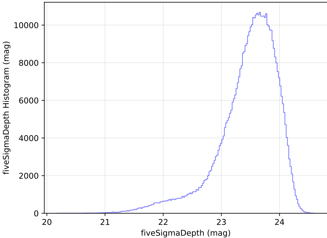
too_elab_r64_d2_ugrizy_v3.4_10yrs i: fiveSigmaDepth Histogram
