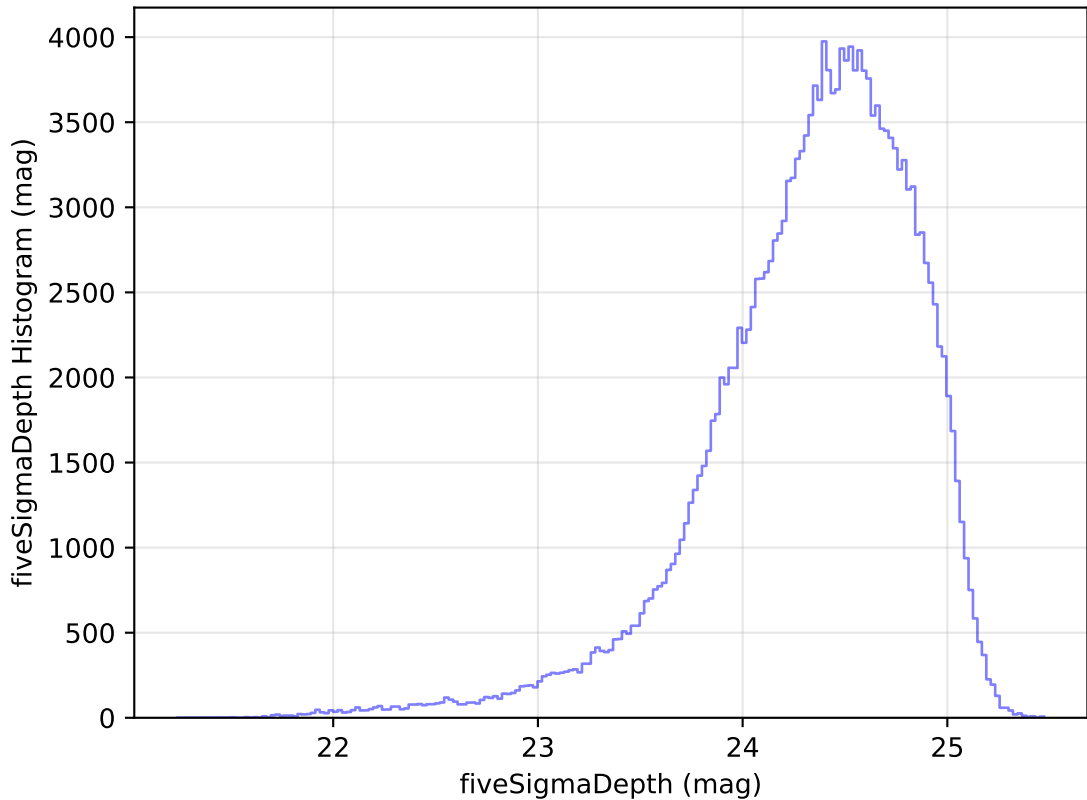
too_elab_r64_d2_ugrizy_v3.4_10yrs g: fiveSigmaDepth Histogram
