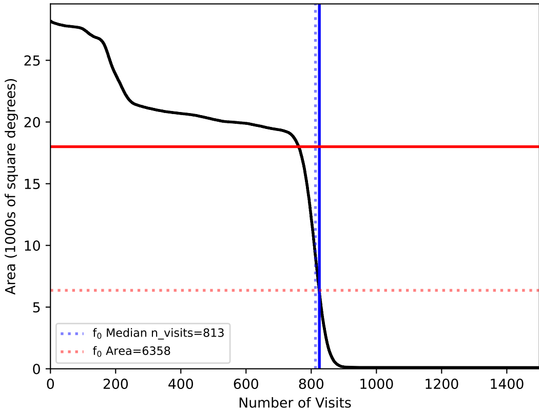
too_elab_r64_d2_ugrizy_v3.4_10yrs : f0
