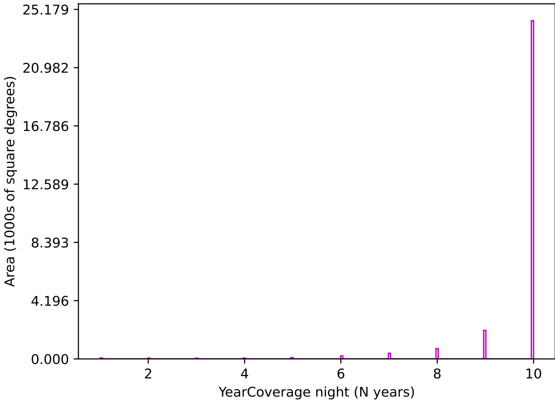
too_elab_r64_d2_ugrizy_v3.4_10yrs z band: YearCoverage night
