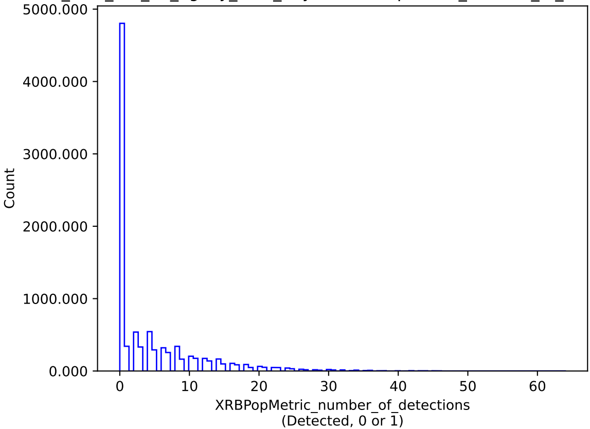
too_elab_r64_d2_ugrizy_v3.4_10yrs : XRBPopMetric_number_of_detections
