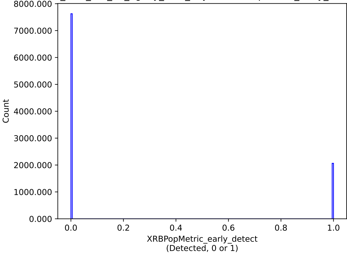
too_elab_r64_d2_ugrizy_v3.4_10yrs : XRBPopMetric_early_detect
