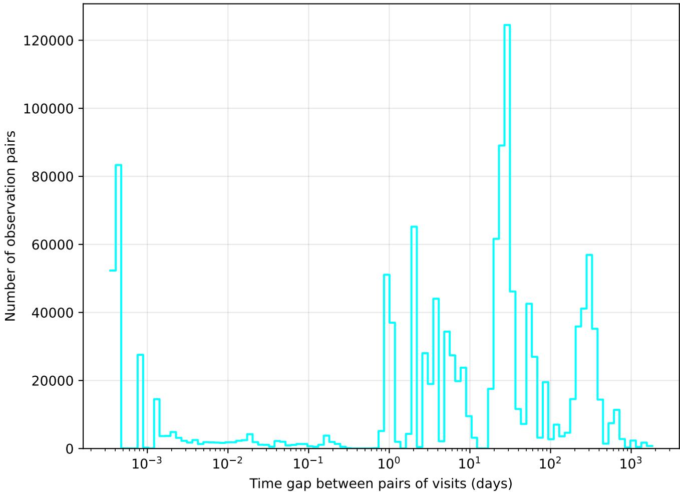
too_elab_r64_d2_ugrizy_v3.4_10yrs u band: Tgaps observationStartMJD
