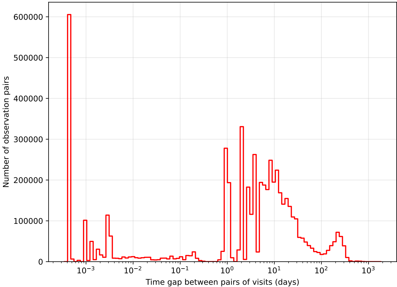
too_elab_r64_d2_ugrizy_v3.4_10yrs i band: Tgaps observationStartMJD
