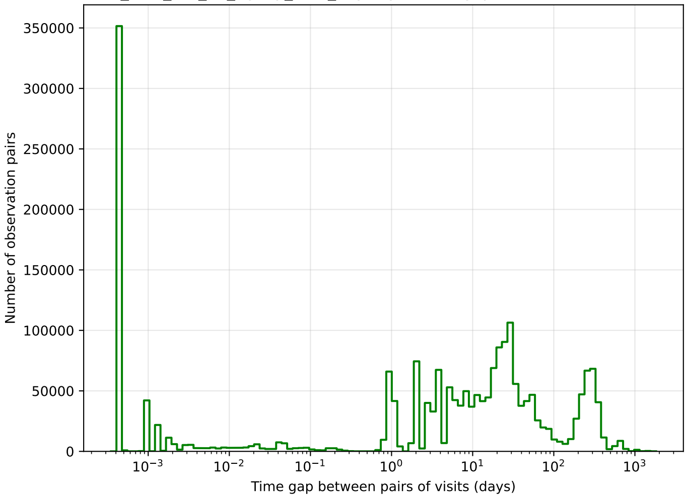
too_elab_r64_d2_ugrizy_v3.4_10yrs g band: Tgaps observationStartMJD
