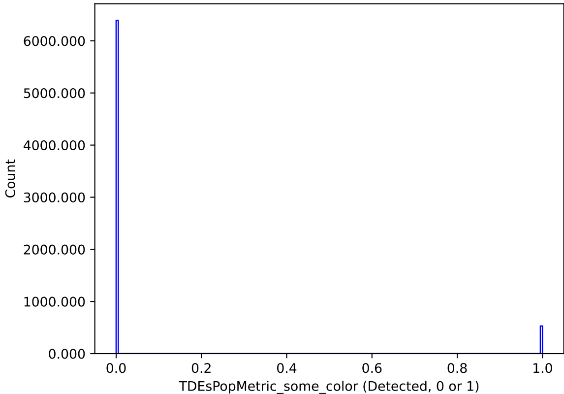
too_elab_r64_d2_ugrizy_v3.4_10yrs : TDEsPopMetric_some_color
