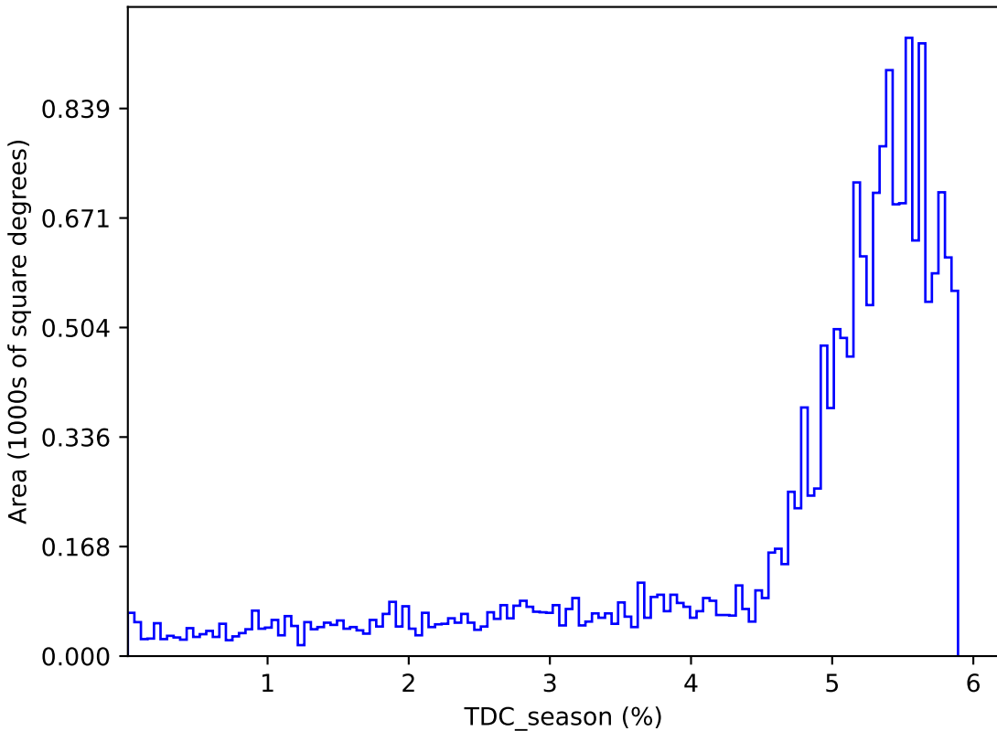
too_elab_r64_d2_ugrizy_v3.4_10yrs : TDC_season
