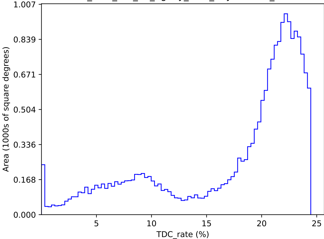
too_elab_r64_d2_ugrizy_v3.4_10yrs : TDC_rate
