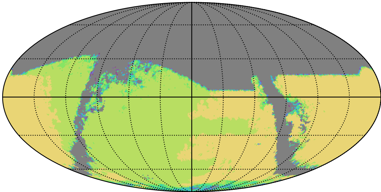
too_elab_r64_d2_ugrizy_v3.4_10yrs : TDC_campaign
