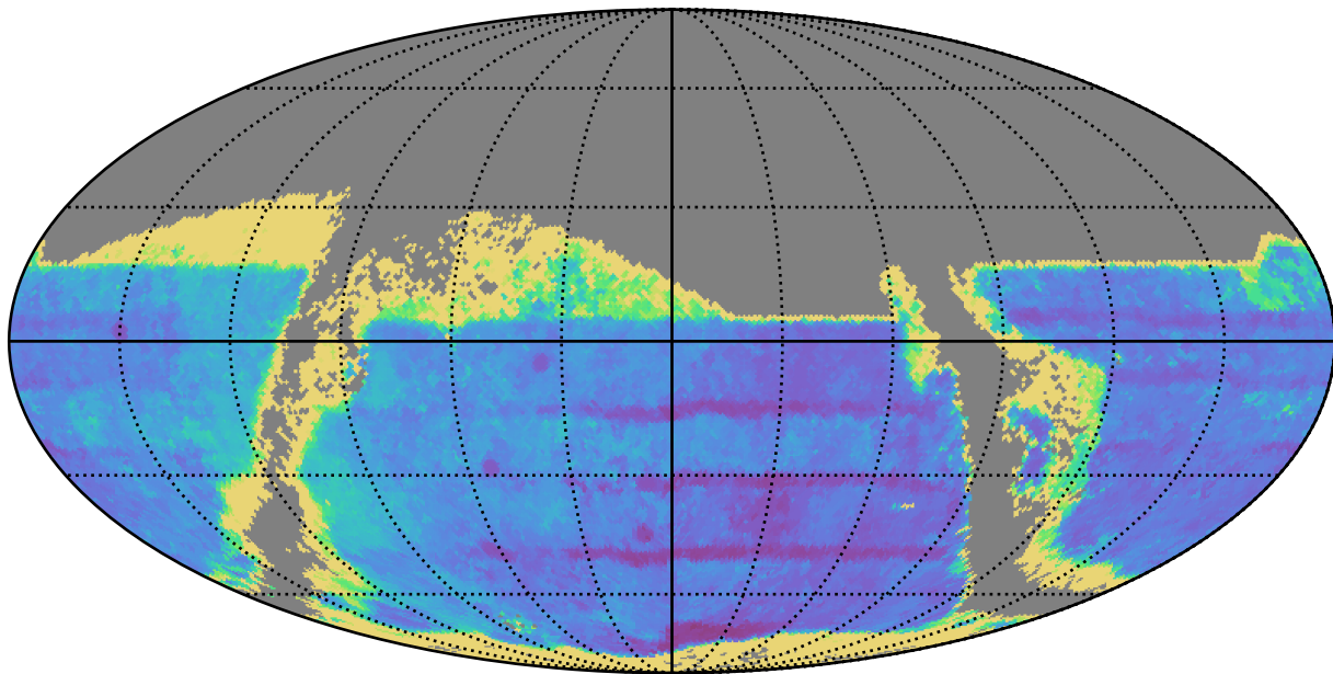
too_elab_r64_d2_ugrizy_v3.4_10yrs : TDC_accuracy
