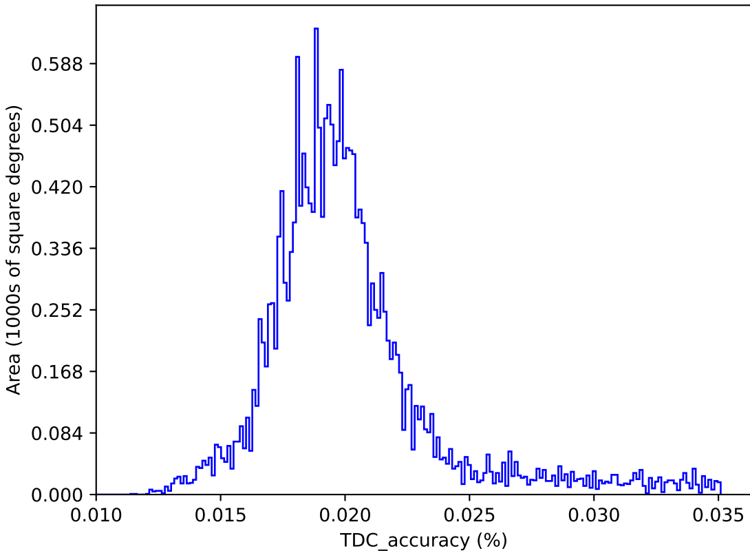
too_elab_r64_d2_ugrizy_v3.4_10yrs : TDC_accuracy
