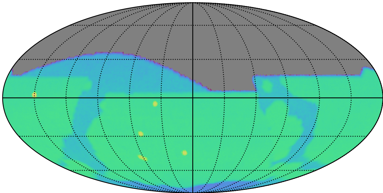
too_elab_r64_d2_ugrizy_v3.4_10yrs r: SurfaceBrightLimit
