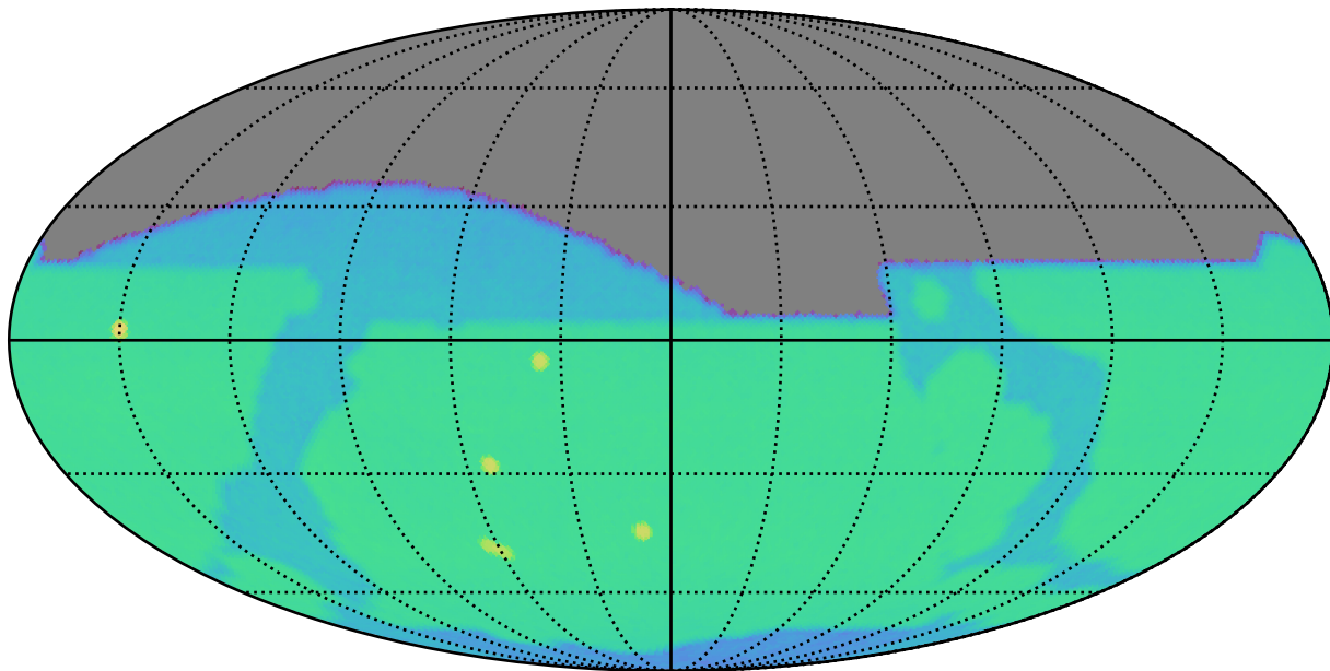
too_elab_r64_d2_ugrizy_v3.4_10yrs i: SurfaceBrightLimit
