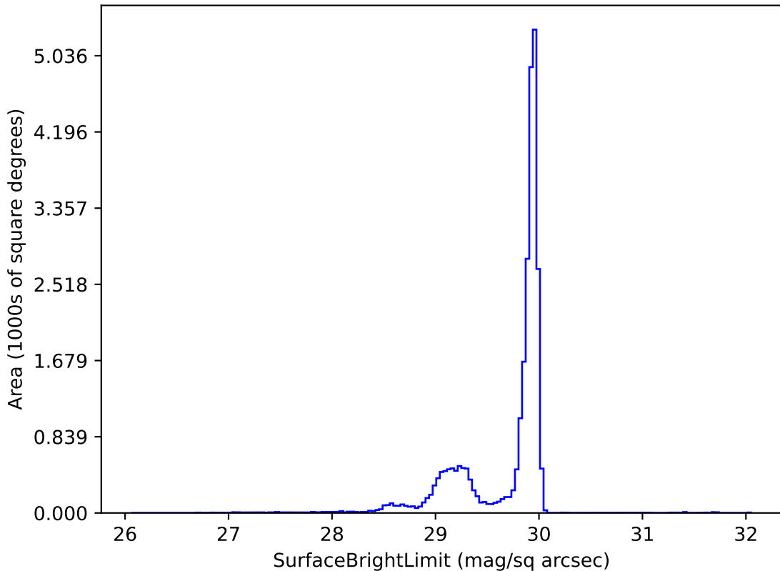
too_elab_r64_d2_ugrizy_v3.4_10yrs i: SurfaceBrightLimit
