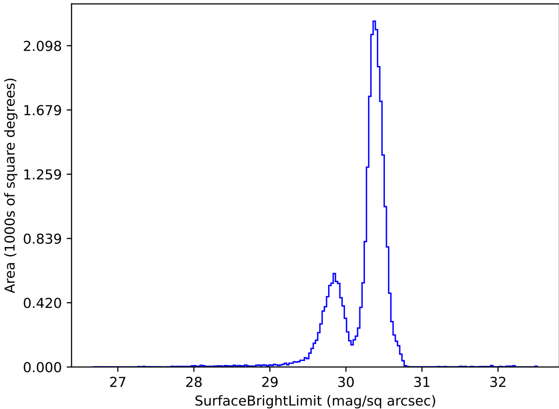
too_elab_r64_d2_ugrizy_v3.4_10yrs g: SurfaceBrightLimit
