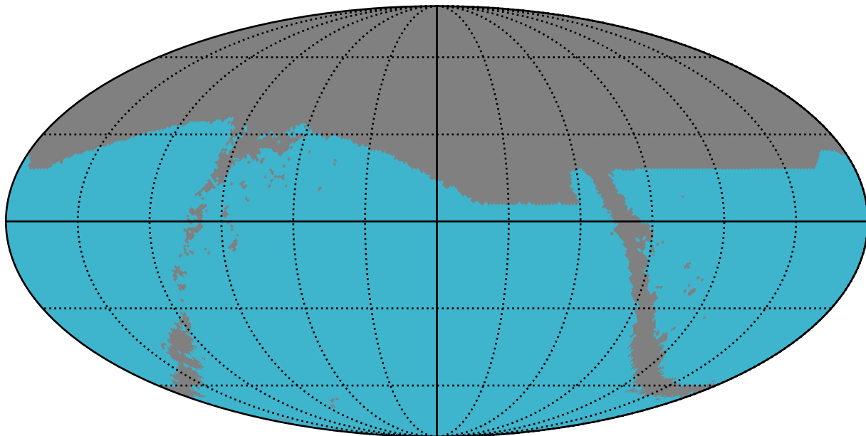
too_elab_r64_d2_ugrizy_v3.4_10yrs : SNSLMetric
