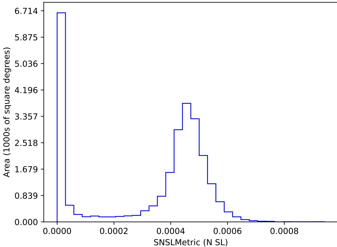
too_elab_r64_d2_ugrizy_v3.4_10yrs : SNSLMetric
