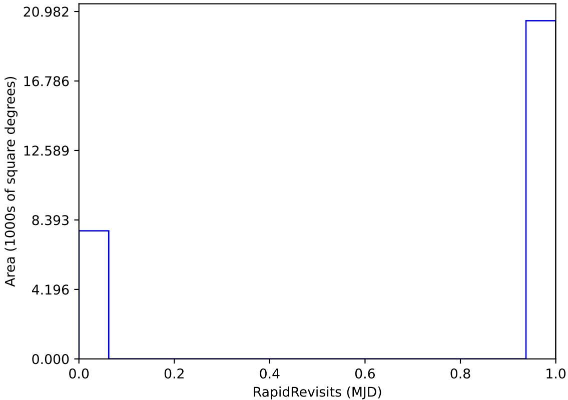
too_elab_r64_d2_ugrizy_v3.4_10yrs : RapidRevisits
