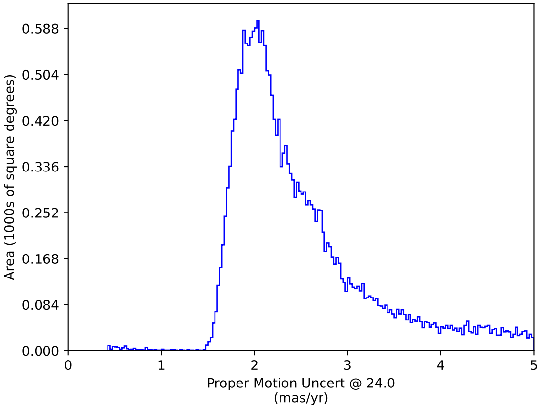
too_elab_r64_d2_ugrizy_v3.4_10yrs : Proper Motion Uncert @ 24.0
